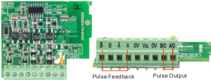
PG Card (EME-PG01)
