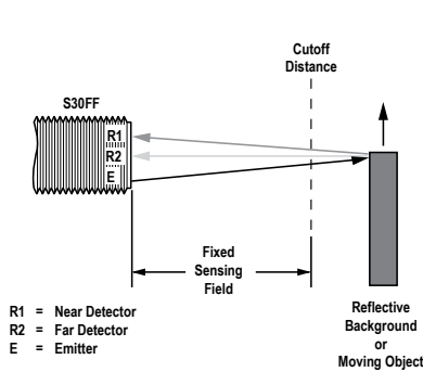
A reflective background object in this position or moving across the sensor face in this axis and direction may cause false sensor response.
