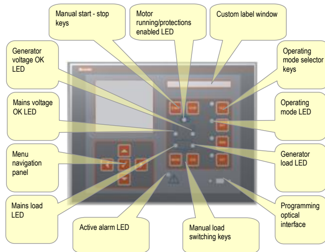
RGK900 front panel
