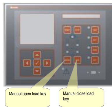
RGK900SA front panel
