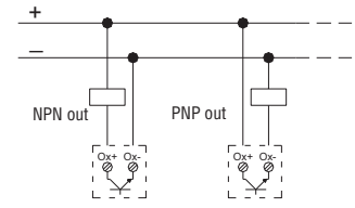
Collegamento uscita impulsi Pulse output connection 30V= - 50mA max
