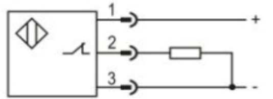
PNP NC
