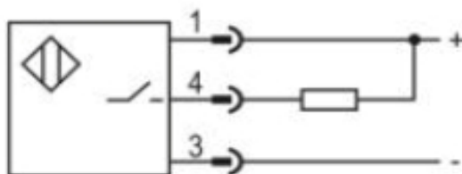
NPN NO
