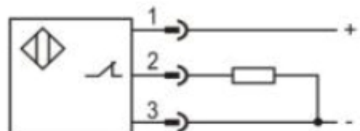
PNP NC
