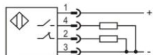
PNP NO+NC
