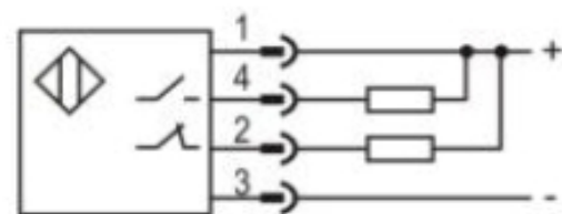
NPN NO+NC
