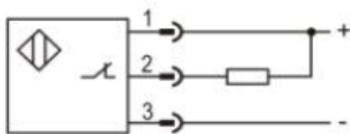
NPN NC
