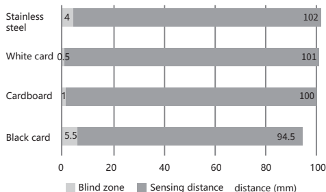
Color sensitivity(PST-YC10*)
