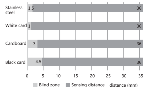
Color sensitivity(PST-YR30*)
