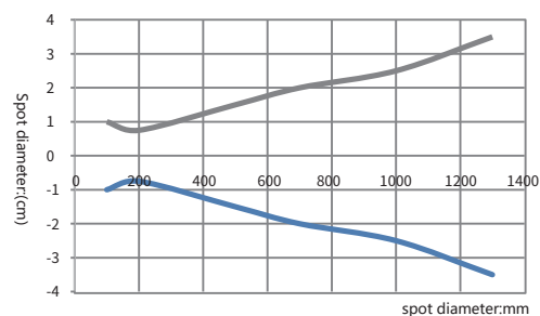
Spot size(PST-TC50*)
