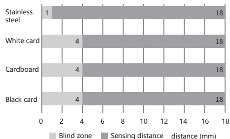
Color sensitivity(PST-YR15*)
