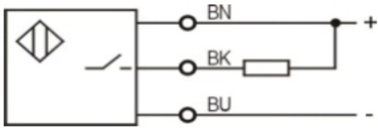
NPN NO
