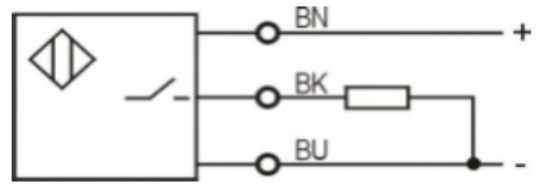
NPN NC
